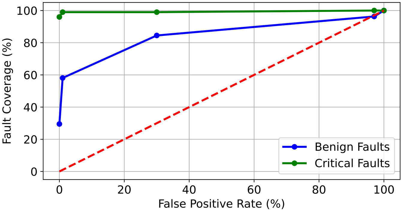
ROC Curve
