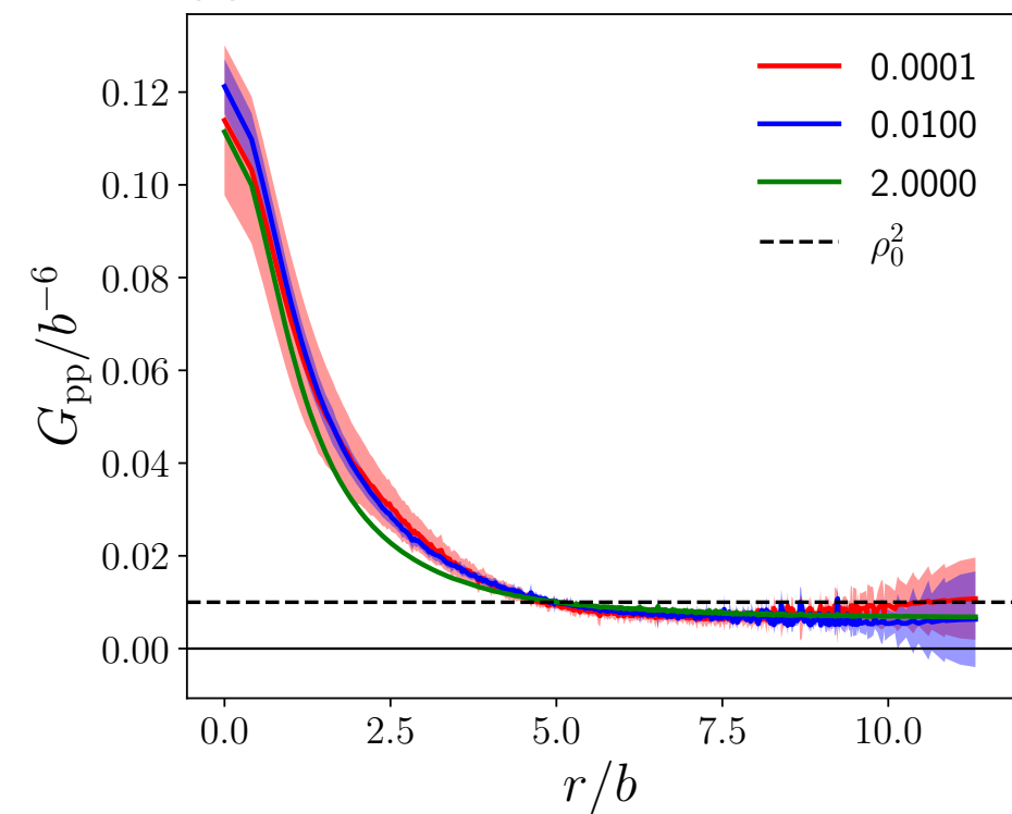
(c) [Na + ] = 10 -4 0.01 2.0
