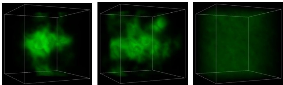
(c) [Na + ] = 10 -4 0.01 2.0
