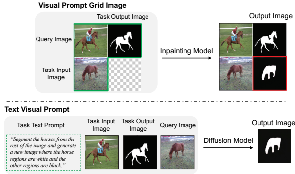
Figure 3: Image-only and textual augmented prompting for visual in-context learning.
