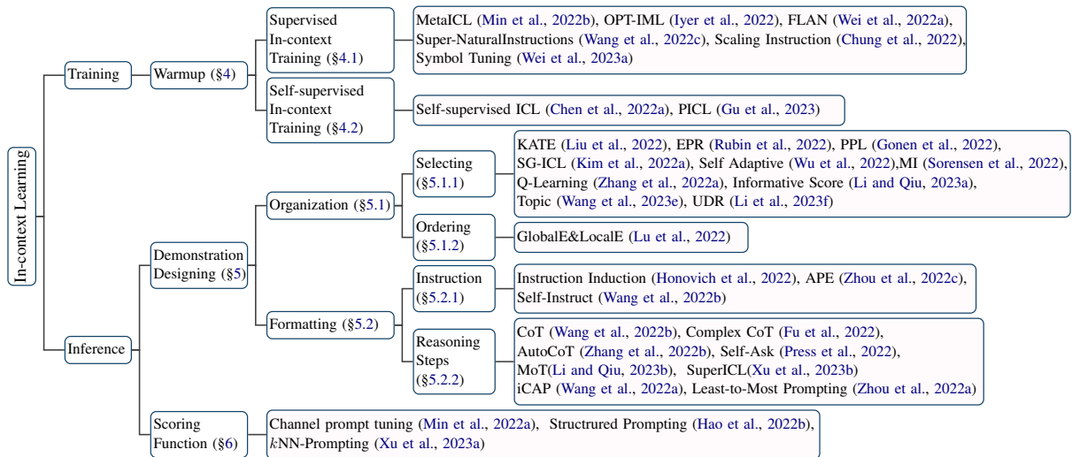
Figure 2: Taxonomy of in-context learning. The training and the inference stage are two main stages for ICL. During the training stage, existing ICL studies mainly take a pretrained LLM as backbone, and optionally warmup the model to strengthen and generalize the ICL ability. Towards the inference stage, the demonstration designing and the scoring function selecting are crucial for the ultimate performance.
