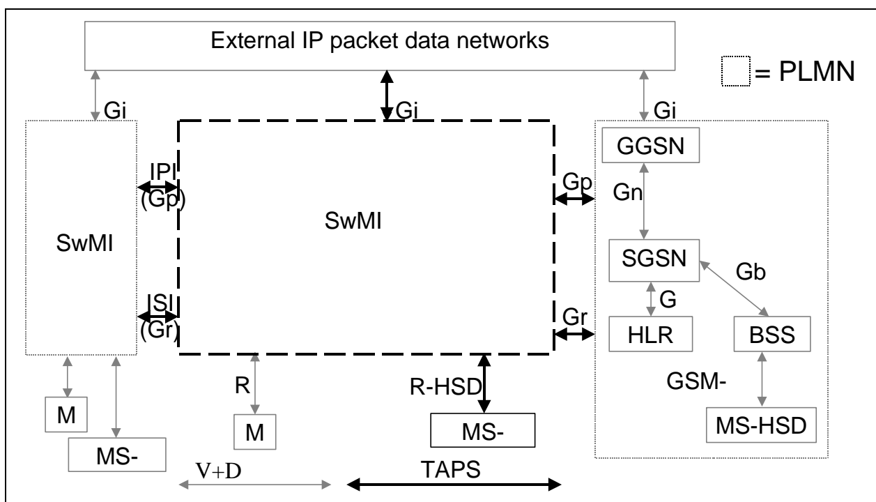
Figure 1: TAPS Interfaces
