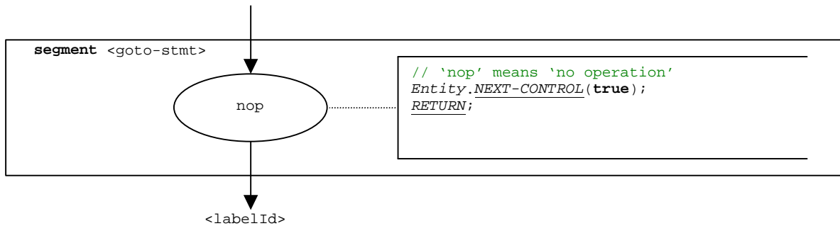
Figure B.80: Flow graph segment <goto-stmt>
