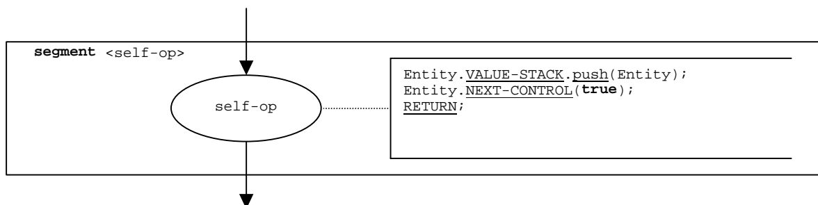
Figure B.109: Flow graph segment <self-op>
