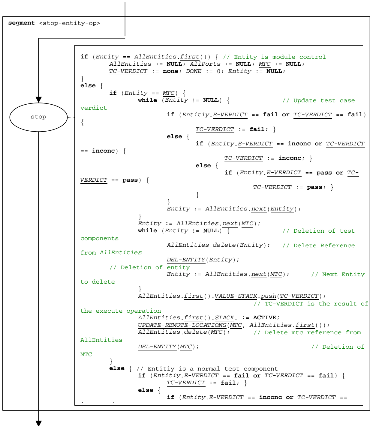
Figure B.116: Flow graph segment &lt;stop-entity-op&gt;
