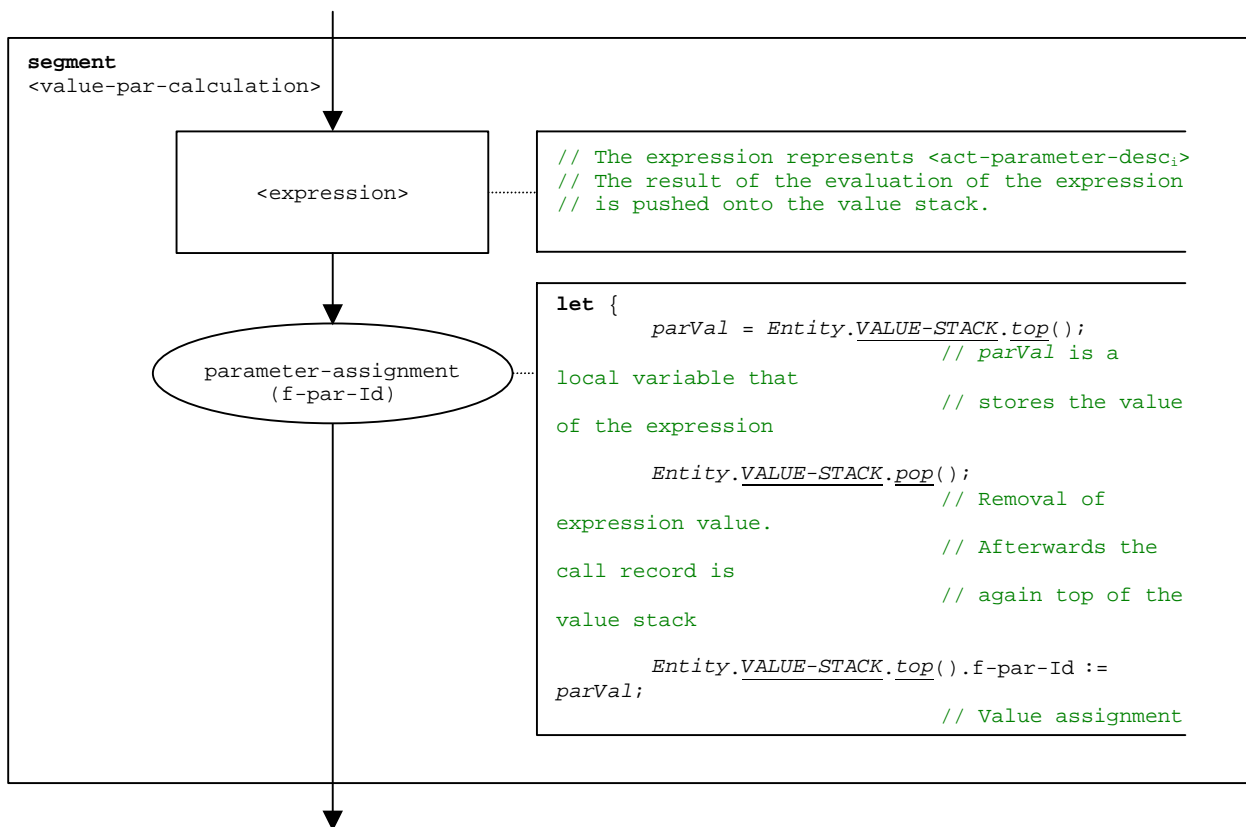
Figure B.70: Flow graph segment <value-par-calculation>
