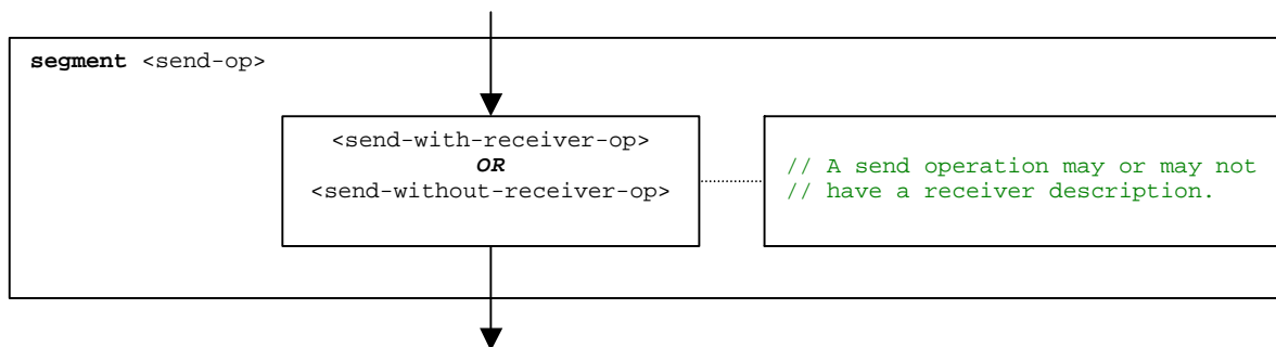
Figure B.106: Flow graph segment <send-op>
