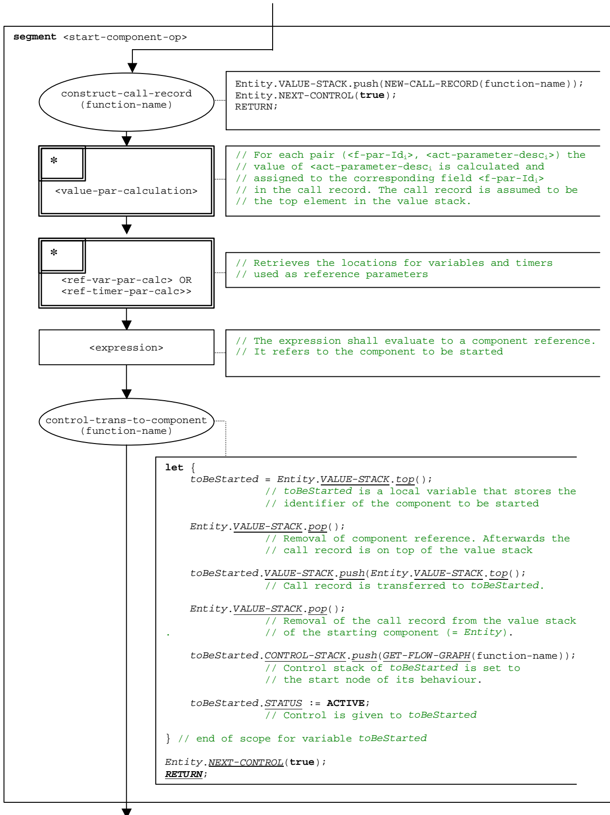
Figure B.110: Flow graph segment &lt;start-component-op&gt;
