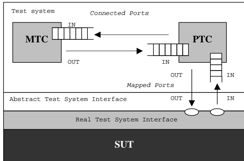
Figure 7: Illustration of the connect and map operations
