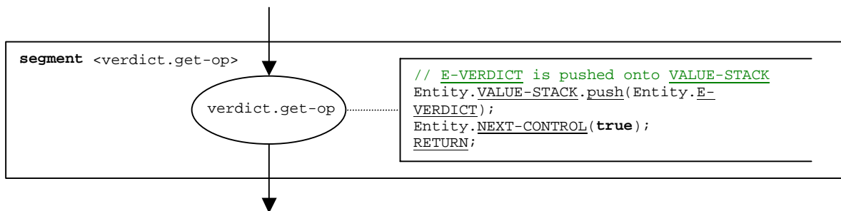
Figure B.123: Flow graph segment <verdict.get-op>
