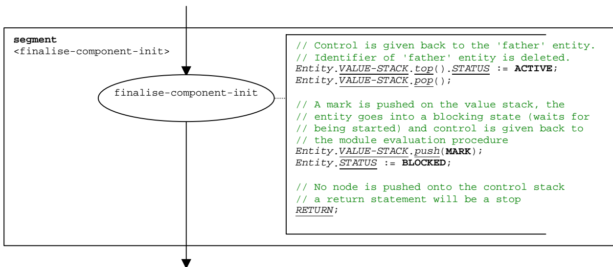
Figure B.66: Flow graph segment <finalize-component-init>
