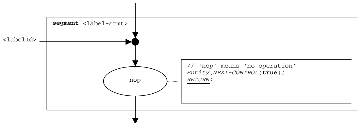
Figure B.84: Flow graph segment <label-stmt>
