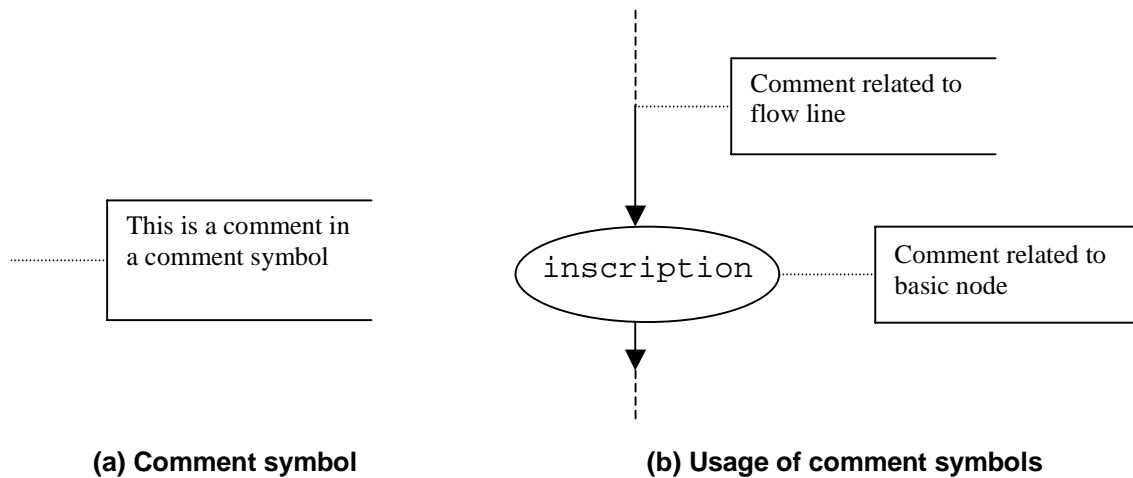
Figure B.9: Flow graph representation of comments
