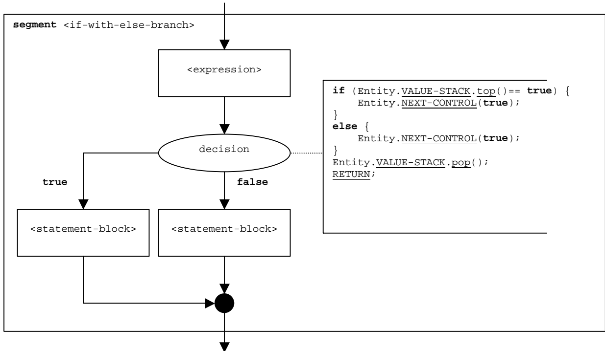
Figure B.82: Flow graph segment <if-with-else-branch>
