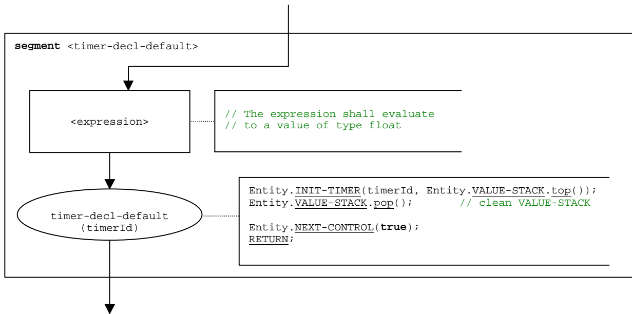
Figure B.48: Flow graph segment <timer-decl-default>
