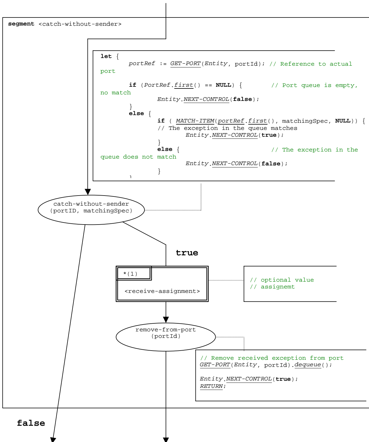
Figure B.41: Flow graph segment <catch-without-sender>
