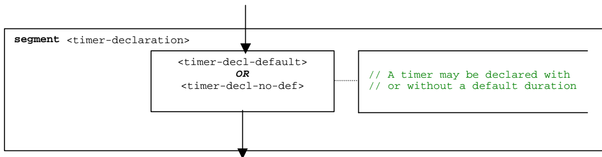
Figure B.47: Flow graph segment <timer-declaration>
