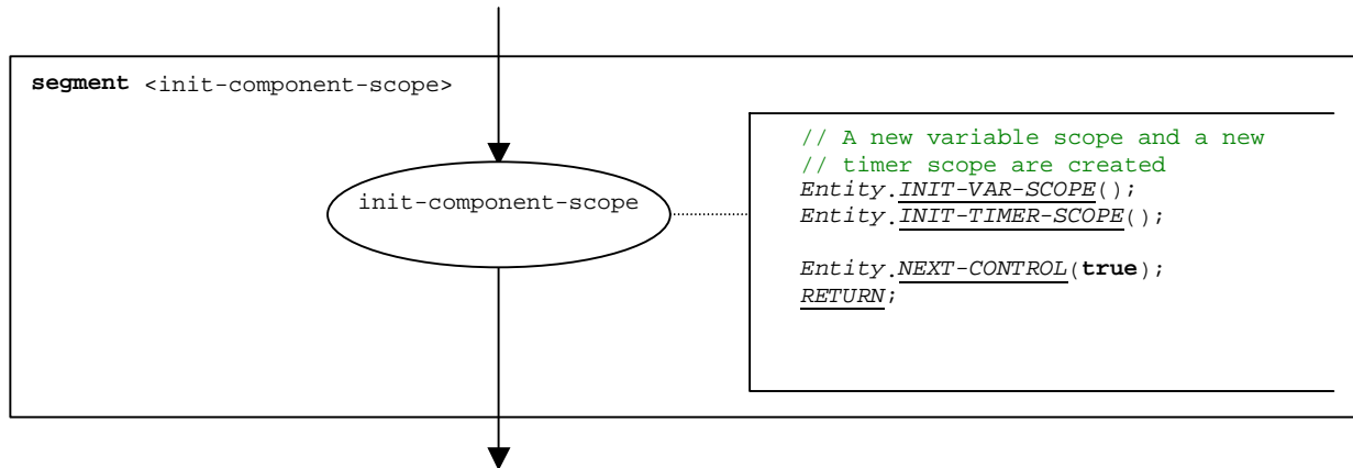
Figure B.67: Flow graph segment <init-component-scope>
