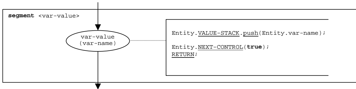
Figure B.63: Flow graph segment <var-value>
