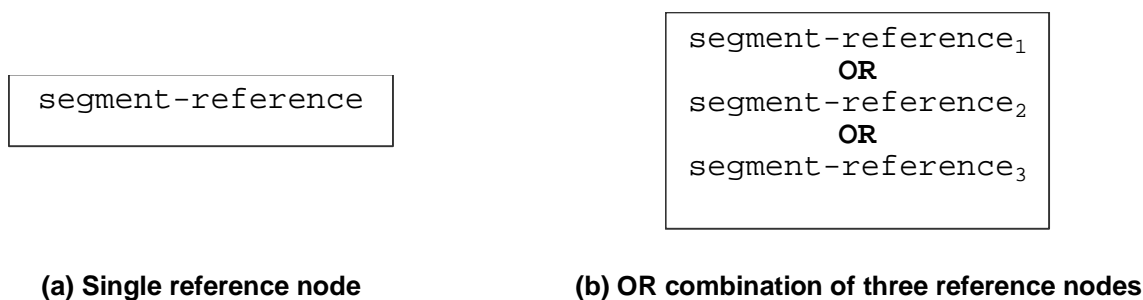
Figure B.5: Reference node
