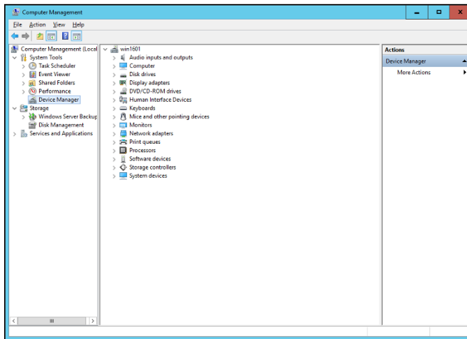
Figure 7-11: Device Manager.
