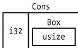
Figure 15-2: A List that is not infinitely sized because Cons holds a Box . Boxes provide only the indirection and heap allocation; they don't have any other special capabilities, like those we'll see with the other smart pointer types. They also don't have any performance overhead that these special capabilities incur, so they can be useful in cases like the cons list where the indirection is the only feature we need. We'll look at more use cases for boxes in Chapter 17 , too.
