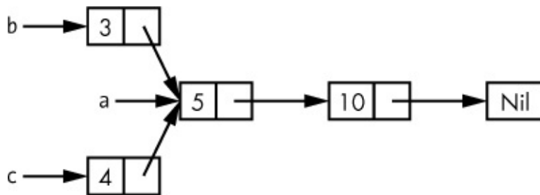
Figure 15-3: Two lists, b and c , sharing ownership of a third list, a . We'll create list a that contains 5 and then 10. Then we'll make two more lists: b that starts with 3 and c that starts with 4. Both b and c lists will then continue on to the first a list containing 5 and 10. In other words, both lists will share the first list containing 5 and 10.
