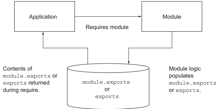
Figure 3.2 The population of the module.exports property or the exports object allows a module to select what should be shared with the application.
