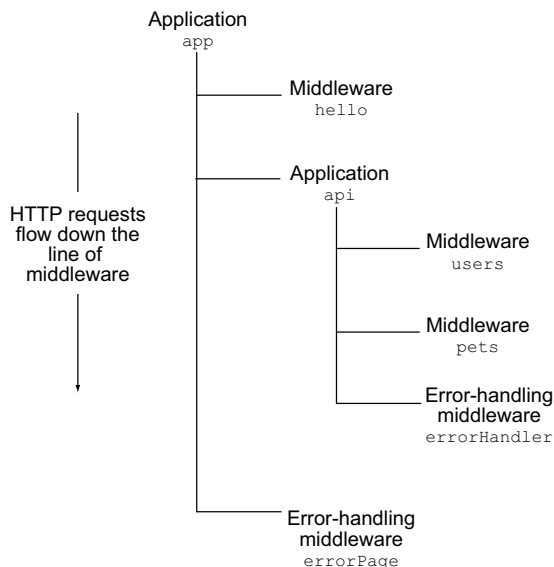
Figure 6.4 Layout of an application with two error-handling middleware components
