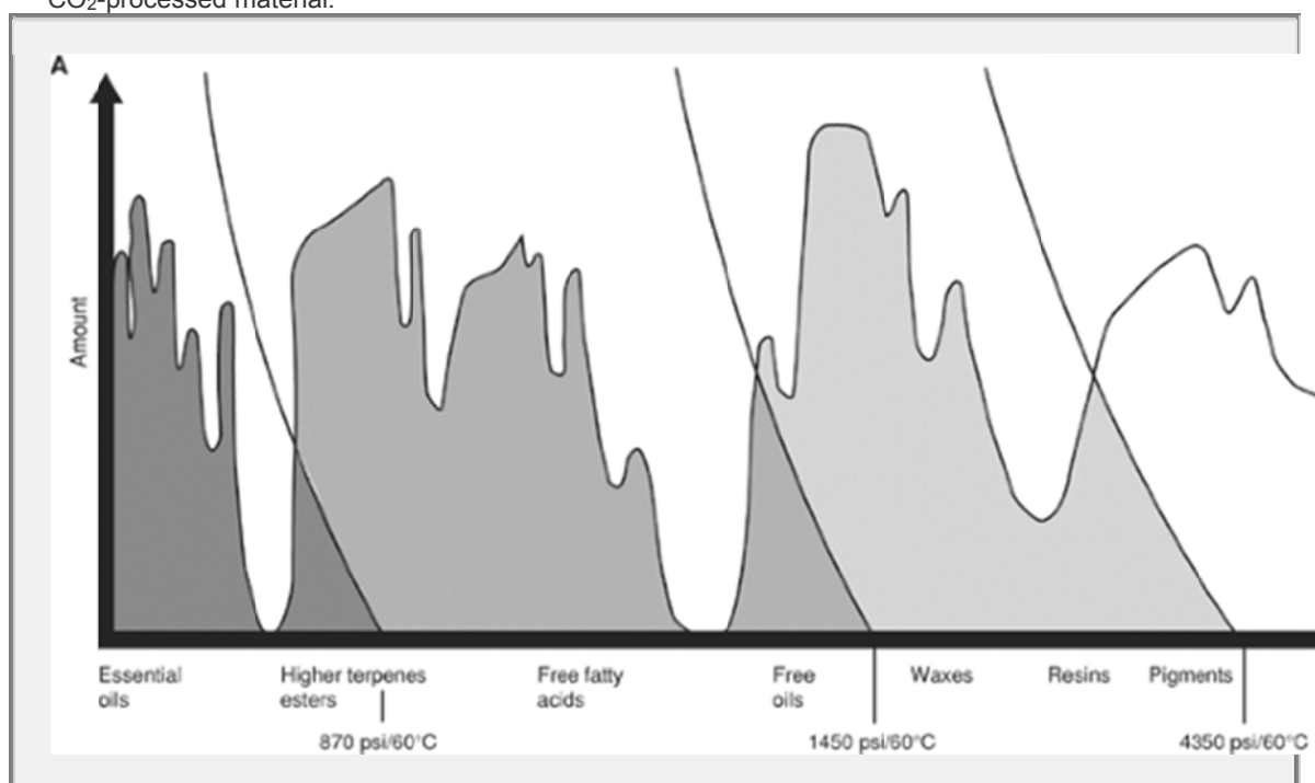
Fig. 2-17. The effect of pressure on the ability of supercritical fluids to selectively extract different compounds. (Modified from Milton Roy Co., Supercritical Fluid Extraction: Principles and Applications [Bulletin 37.020], Milton Roy Co., Ivyland, Pa.)
