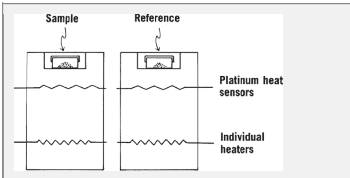
Fig. 2-21. Separate heat sources and platinum heat sensors used in differential scanning calorimetry.
