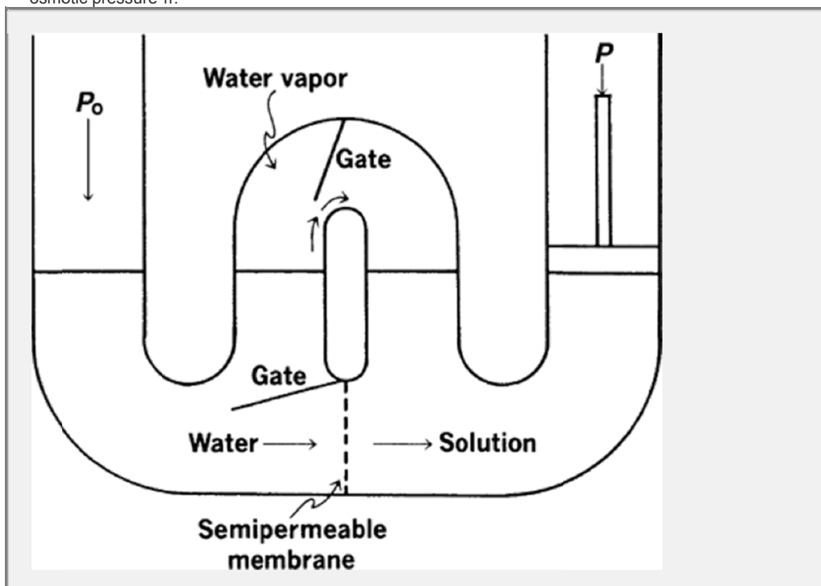
Fig. 5-12. Apparatus for demonstrating the relationship between osmotic pressure and vapor pressure lowering.
