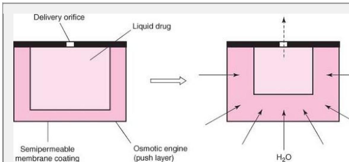
Fig. 23-22. Schematic representation of L-OROS osmotic drug delivery system. The drug is liberated through the small orifice due to the osmosis of fluids through the semipermeable membrane into the osmotic push layer.
