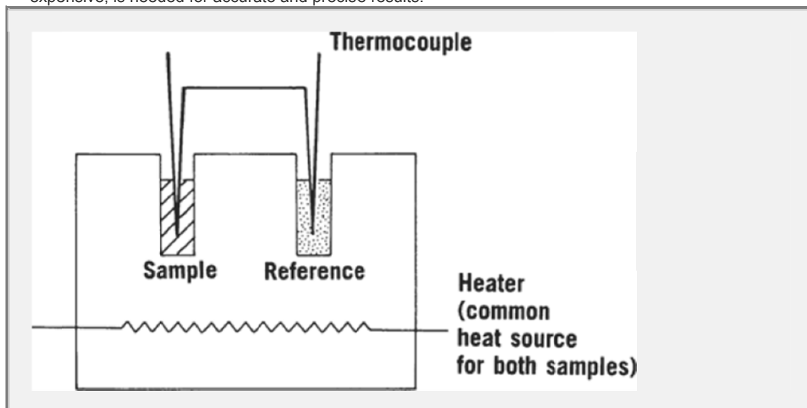
Fig. 2-20. Common heat source of differential thermal analyzer with thermocouples in contact with the sample and the reference material.
