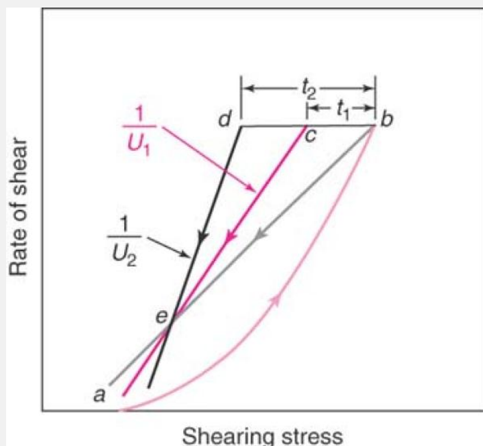
Fig. 19-5. Structural breakdown with time of a plastic system possessing thixotropy when subjected to a constant rate of shear for t_1 and t_2 seconds. See text for discussion.
