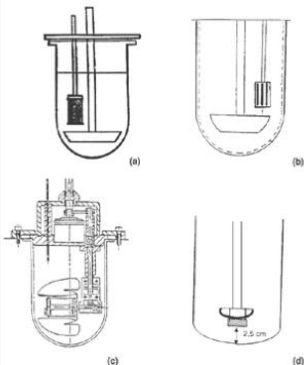
Basket apparatus No stirring
