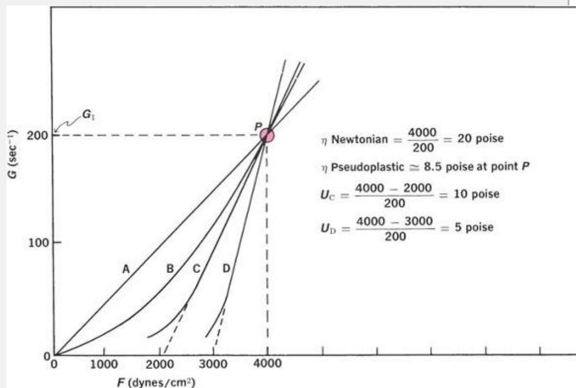
Fig. 19-10. Errors inherent in the use of a "one-point" instrument for non-Newtonian systems. Regardless of the fact that A is Newtonian, B is pseudoplastic, and C and D
