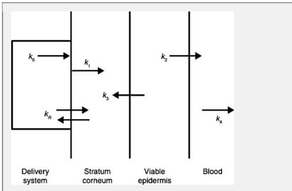
Fig. 23-30. Transdermal delivery of clonidine from a membrane-controlled patch. (Modified from R. H. Guy and J. Hadgraft, J Pharm. Sci. 74 , 1016, 1985. With permission.)
