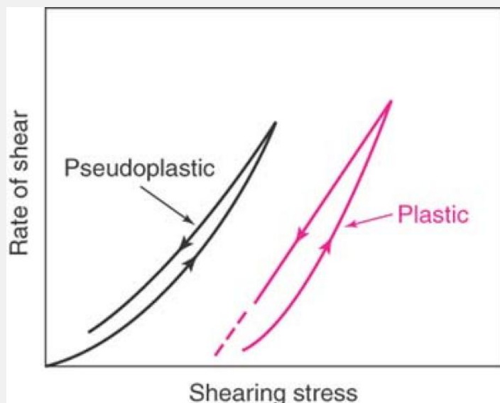
Fig. 19-4. Thixotropy in plastic and pseudoplastic flow systems.
