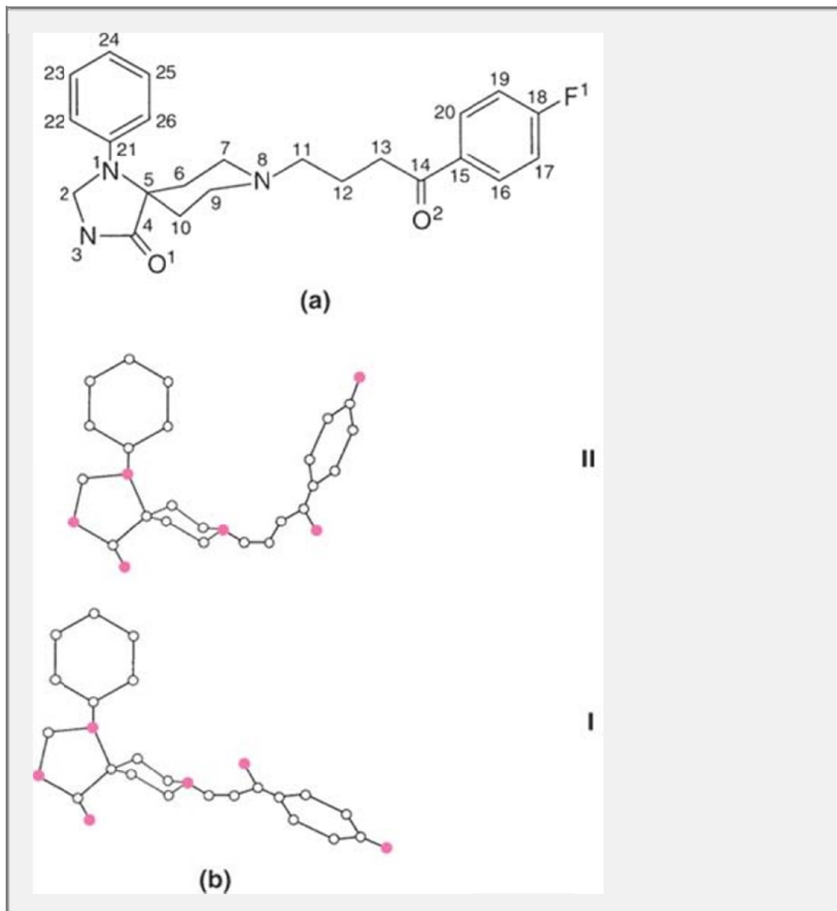
Fig. 2-7. (a) Structure and numbering of spiperone. (b) Molecular conformation of two polymorphs, I and II, of spiperone. (Modified from J. W. Moncrief and W. H. Jones, Elements of Physical Chemistry , Addison-Wesley, Reading, Mass., 1977, p. 93; R. Chang, Physical Chemistry with Applications to Biological Systems , 2nd Ed., Macmillan, New York, 1977, p. 162.) (From M. Azibi, M. Draguet-Brughmans, R. Bouche, B. Tinant, G. Germain, J. P. Declercq, and M. Van Meerssche, J. Pharm. Sci. 72 , 232, 1983. With permission.)
