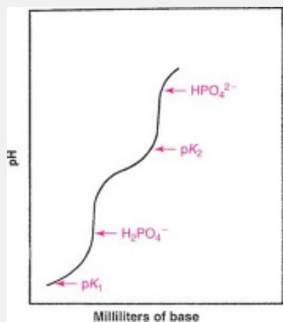
Fig. 8-2. Neutralization of a tribasic acid.
