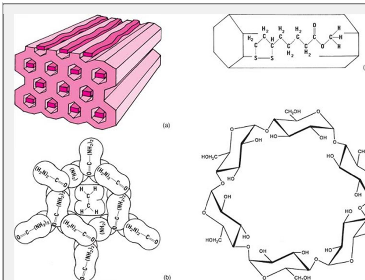
Fig. 10-3. (a) A channel complex formed with urea molecules as the host. (b) These molecules are packed in an orderly manner and held together by hydrogen bonds between nitrogen and oxygen atoms. The hexagonal channels, approximately 5 Å in diameter, provide room for guest molecules such as long-chain hydrocarbons, as shown here. (From J. F. Brown, Jr., Sci. Am. 207 , 82, 1962. Copyright © 1962 by Scientific American, Inc. All rights reserved.) (c) A hexagonal channel complex (adduct) of methyl \alpha -lipoate and 15 g of urea in methanol prepared with gentle heating. Needle crystals of the adduct separated overnight at room temperature. This inclusion compound or adduct begins to decompose at 63°C and melts at 163°C. Thiourea may also be used to form the channel complex. (From H. Mina and M. Nishikawa, J. Pharm. Sci. 53 , 931, 1964. With permission.) (d) Cyclodextrin (cycloamylose, Schardinger dextrin). (See Merck Index , 11th Ed., Merck, Rahway, N.J., 1989, p. 425.)
