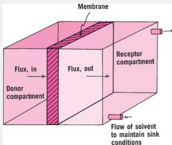
Fig. 11-3. Diffusion cell. The donor compartment contains diffusant at concentration C .
