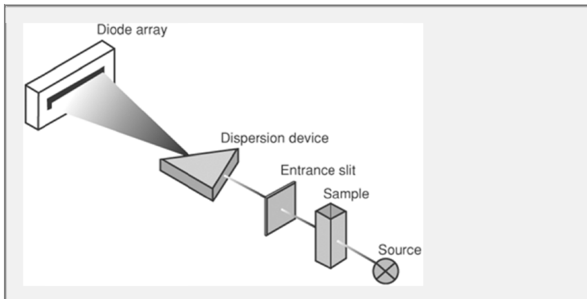
Fig. 4-9. Schematic of an HP-8453 diode-array ultraviolet–visible spectrophotometer. (Courtesy of Hewlett-Packard, Palo Alto, CA.)
