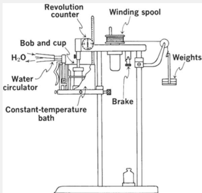
Fig. 19-16. Stormer viscometer. The falling weights cause the bob to rotate in the stationary cup. The velocity of the bob is obtained by means of a stopwatch and the
