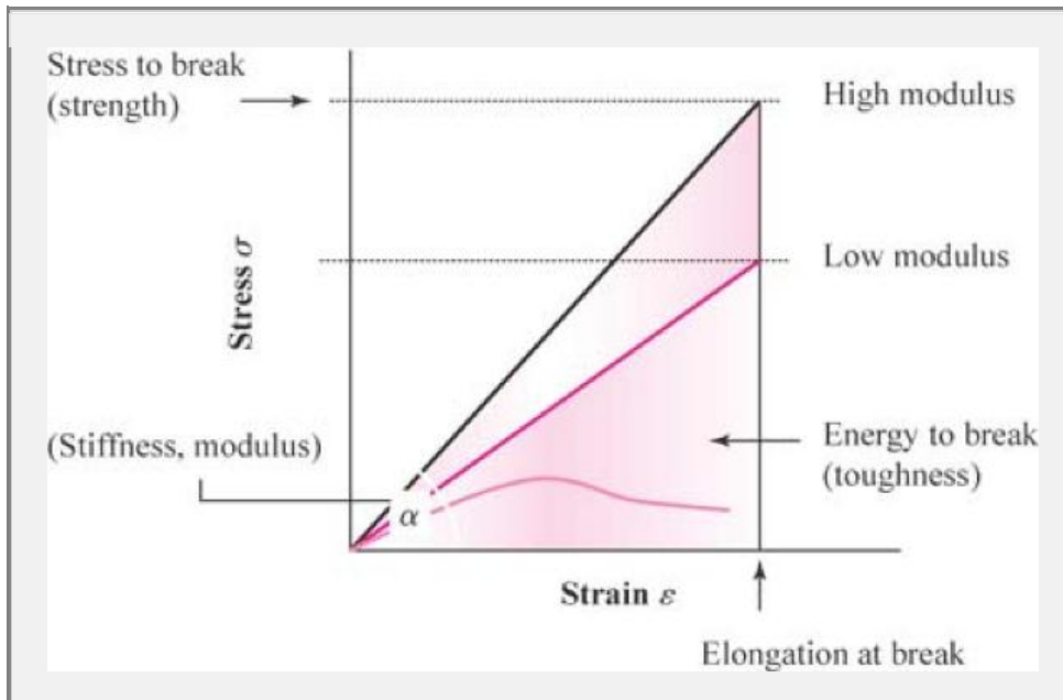
Fig. 20-11. Mechanical properties of polymers.
