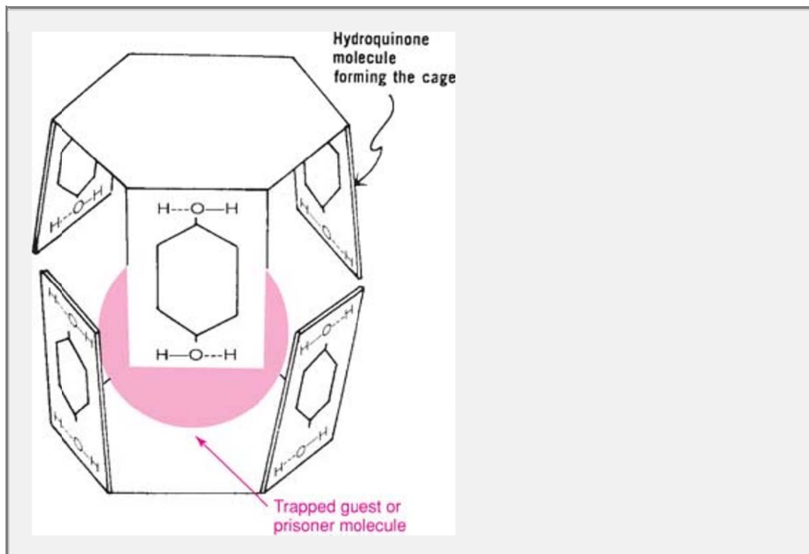
Fig. 10-4. Cagelike structure formed through hydrogen bonding of hydroquinone molecules. Small molecules such as methanol are trapped in the cages to form the clathrate. (Modified from J. F. Brown, Jr., Sci. Am. 207 , 82, 1962. Copyright © 1962 by Scientific American, Inc. All rights reserved.)
