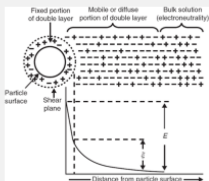
Fig. 16-11. Diffuse double layer and the zeta potential.
