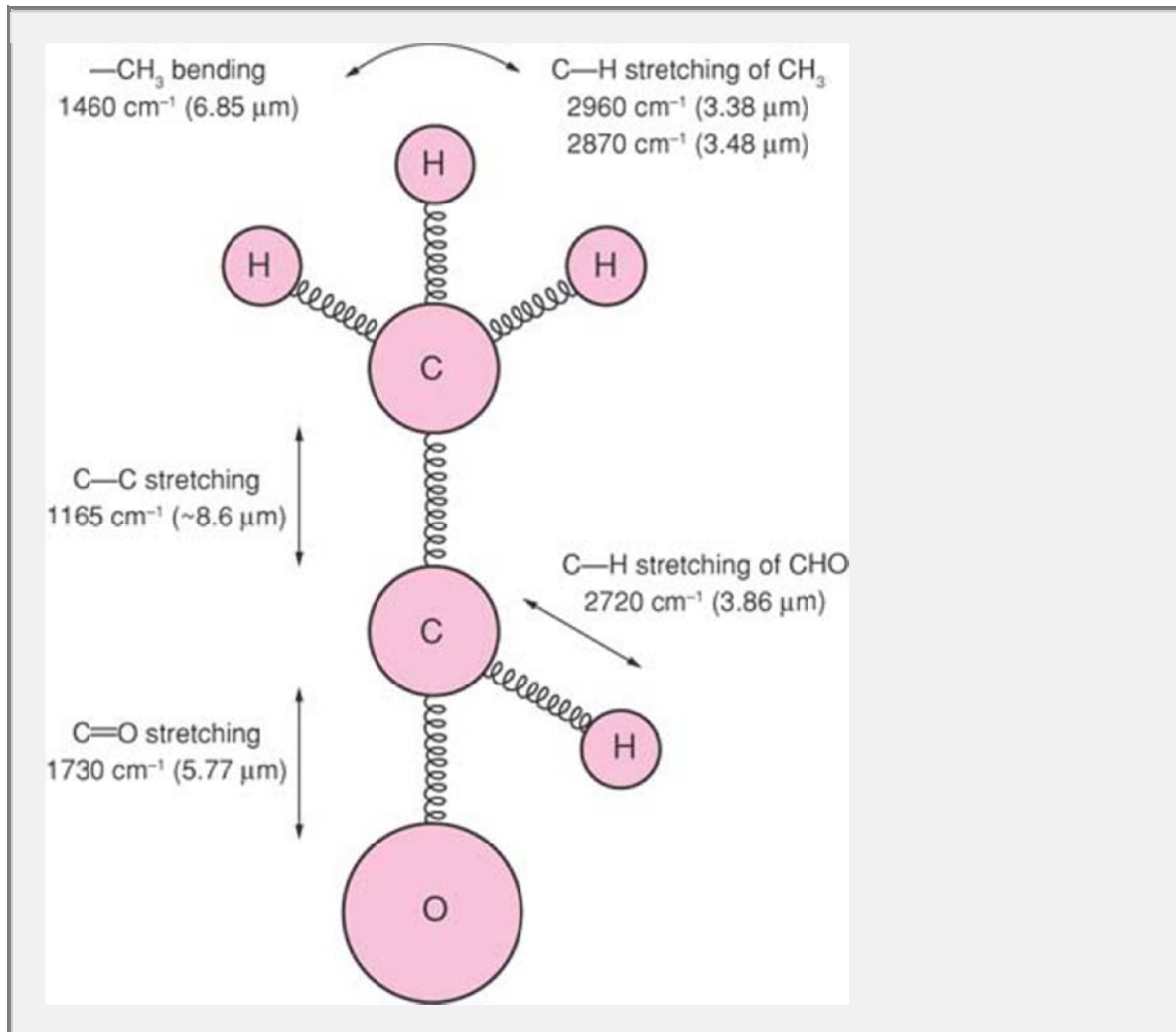
Fig. 4-14. Bending and stretching frequencies for acetaldehyde. (From H. H. Willard, L. L. Merritt, Jr., and J. A. Dean, Instrumental Methods of Analysis , 4th Ed., Van Nostrand, New York, 1968. With permission.)
