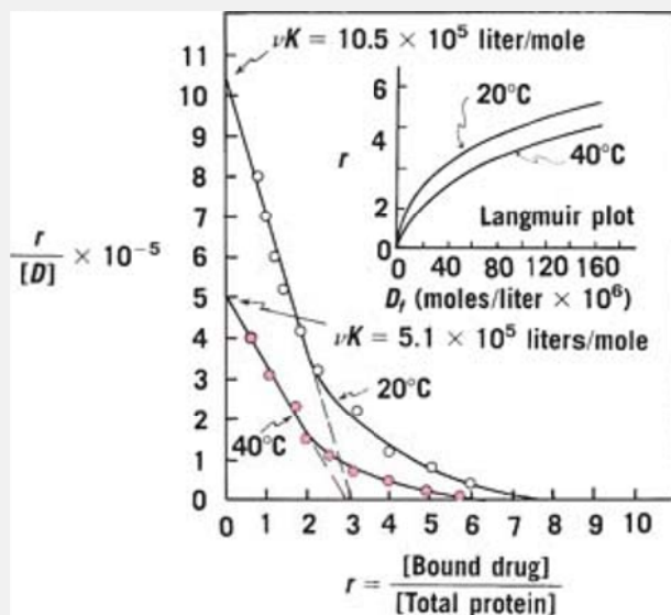
Fig. 10-17. A Scatchard plot showing the binding of bishydroxycoumarin to human serum albumin at 20°C and 40°C plotted according to equation(10-41). Extrapolation of the two lines to the horizontal axis, assuming a single class of sites with no electrostatic interaction, gives an approximate value of 3 for v . (From M. J. Cho, A. G. Mitchell, and M. Pernarowski, J. Pharm. Sci. 60 , 196, 1971; 60 , 720, 1971. With permission.) The inset is a Langmuir adsorption isotherm of the binding data plotted according to equation(10-36).
