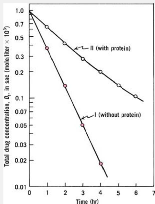
Fig. 10-18. The dynamic dialysis plot for determining the concentration of bound drug in a protein solution (From M. C. Meyer and D. E. Guttman, J. Pharm. Sci. 57 , 1627, 1968. With permission).
