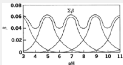
Fig. 8-5. The total buffer capacity of a universal buffer as a function of a pH. (From I. M. Kolthoff and C. Rosenblum, Acid-Base Indicators , Macmillan, New York, 1937, p. 29.)
