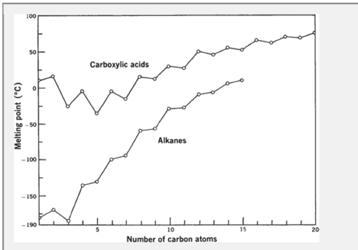
Fig. 2-13. The melting points of alkanes and carboxylic acids as a function of carbon chain length. (Modified from C. R. Noller, Chemistry of Organic Compounds , 2nd Ed., Saunders, Philadelphia, 1957, pp. 40, 149.)
