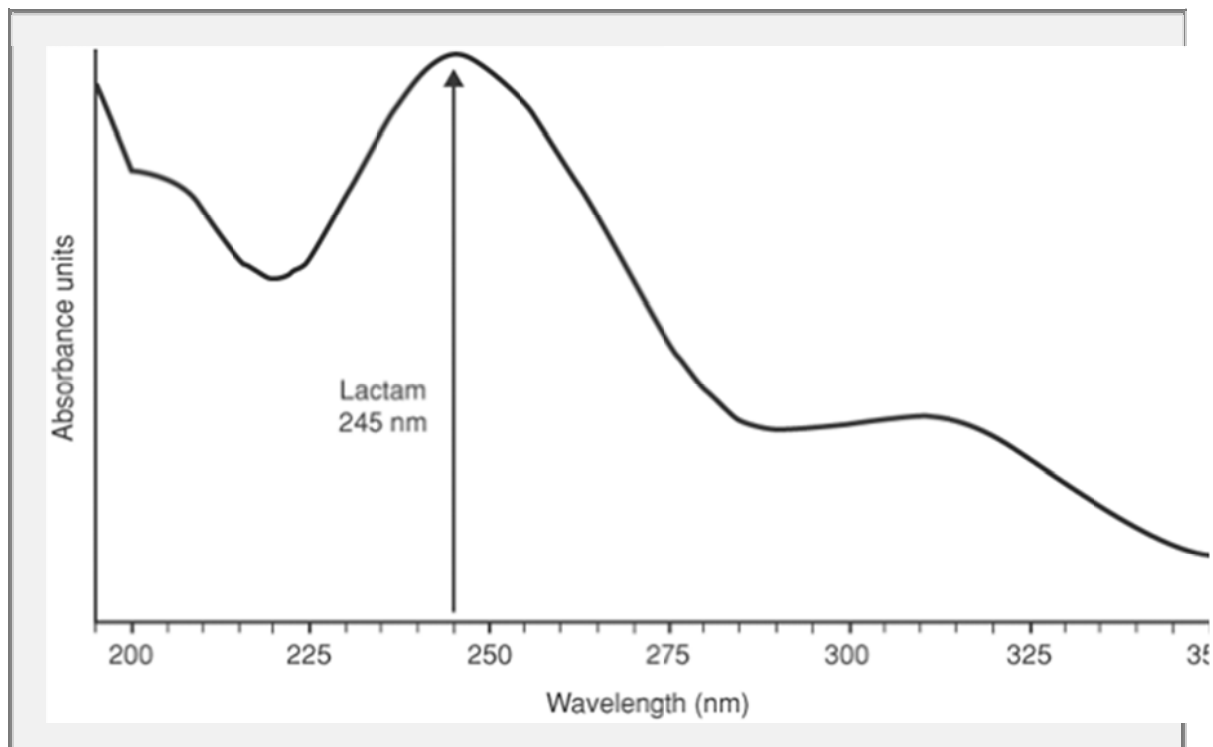
Fig. 4-8. The absorbance maxima of chlordiazepoxide lactam as a function of the wavelength. (Modified from http://chrom.tutms.tut.ac.jp/JINNO/DRUGDATA/17chlordia-zepoxide.html )
