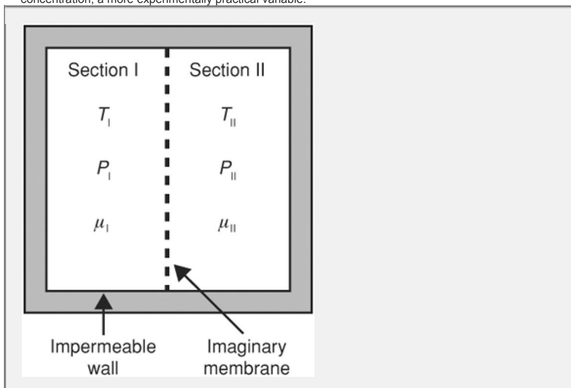
Fig. 11-2. Isolated system consisting of two sections separated by an imaginary permeable membrane. At equilibrium, the temperatures ( T ), pressures ( P ), and chemical properties ( \mu ) of each of the species in the system are equal in the two sections. (Modified from G. L. Amidon, P. I. Lee, and E. M. Topp (Eds.), Transport Processes in Pharmaceutical Systems , Marcel Dekker, New York, 2000, p. 13.) 84
