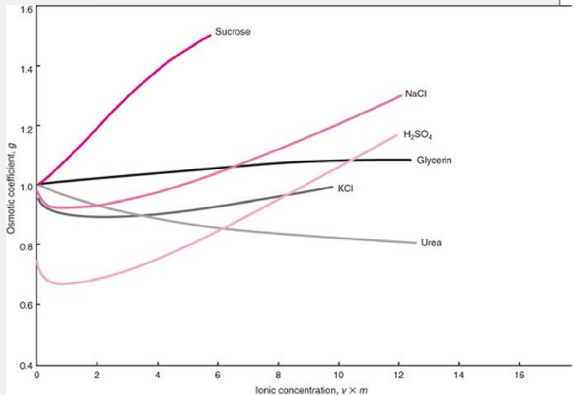
Fig. 6-8. Osmotic coefficient, g , for some common solutes. (From G. Scatchard, W.
