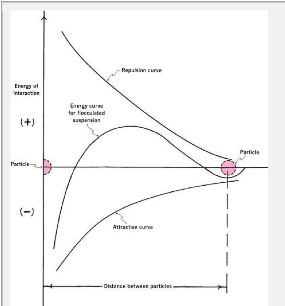
Fig. 17-1. Potential energy curves for particle interactions in suspension. (From A. Martin, J. Pharm. Sci. 50 , 514, 1961. With permission.)
