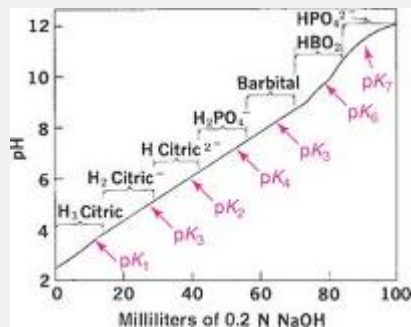
Fig. 8-3. Neutralization curve for a universal buffer. (From H. T. Britton, Hydrogen Ions , Vol. I, Van Nostrand, New York, 1956, p. 368.)
