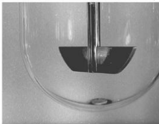
Paddle apparatus No stirring
