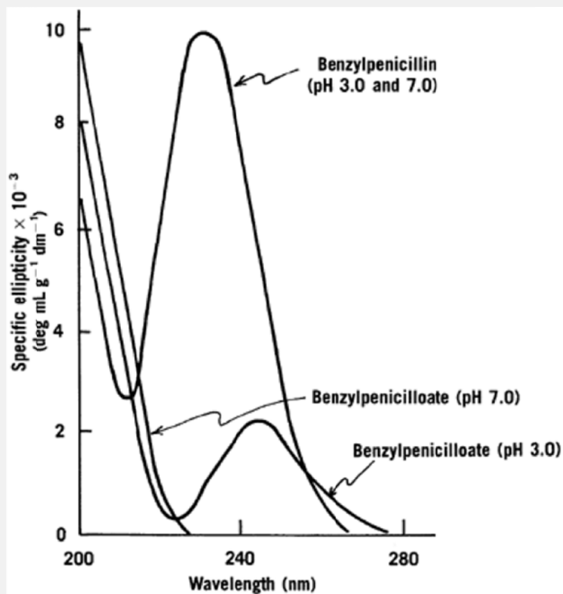
Fig. 4-27. Circular dichroism spectra of benzylpenicillin and its penicilloic acid derivative. (From C. E. Rassmussen and T. Higuchi, J. Pharm. Sci. 60 , 1616, 1971. With permission.)
