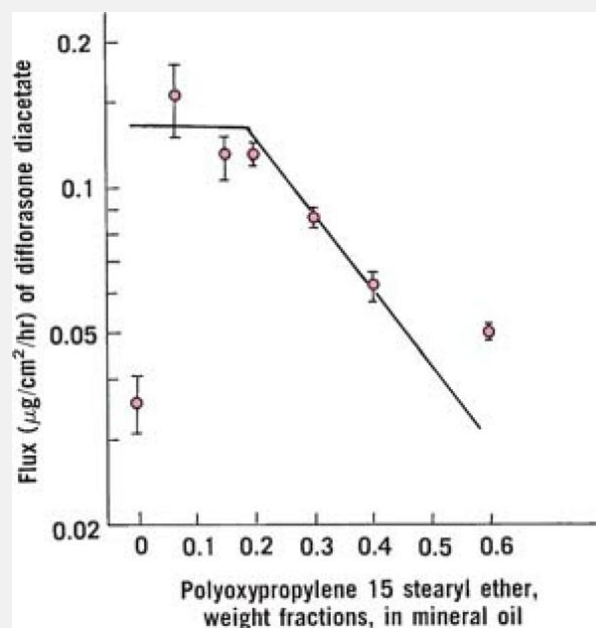
Fig. 11-19. Steady-state flux of diflorasone diacetate in a mixture of polyoxypropylene 15 stearyl ether in mineral oil. (From J. S. Turi, D. Danielson, and W. Woltersen, J. Pharm. Sci. 68 ,275, 1979. With permission.)
